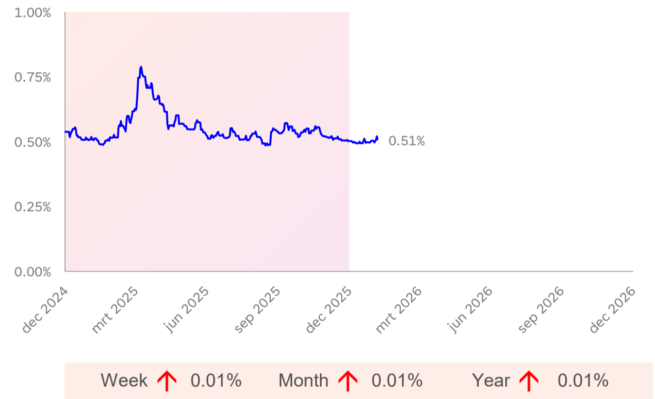
Figure 2: Credit risk
