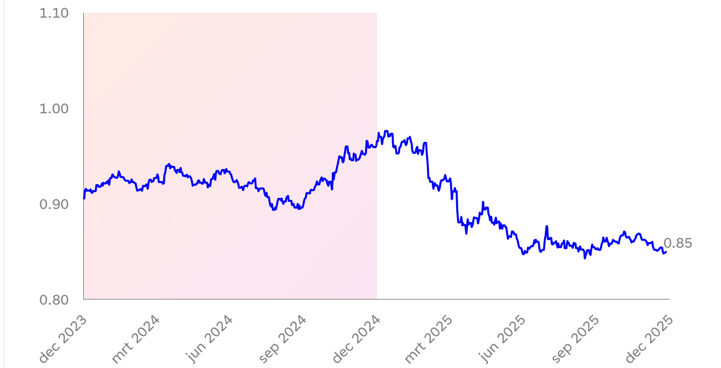
Figure 6: US Dollar risk
