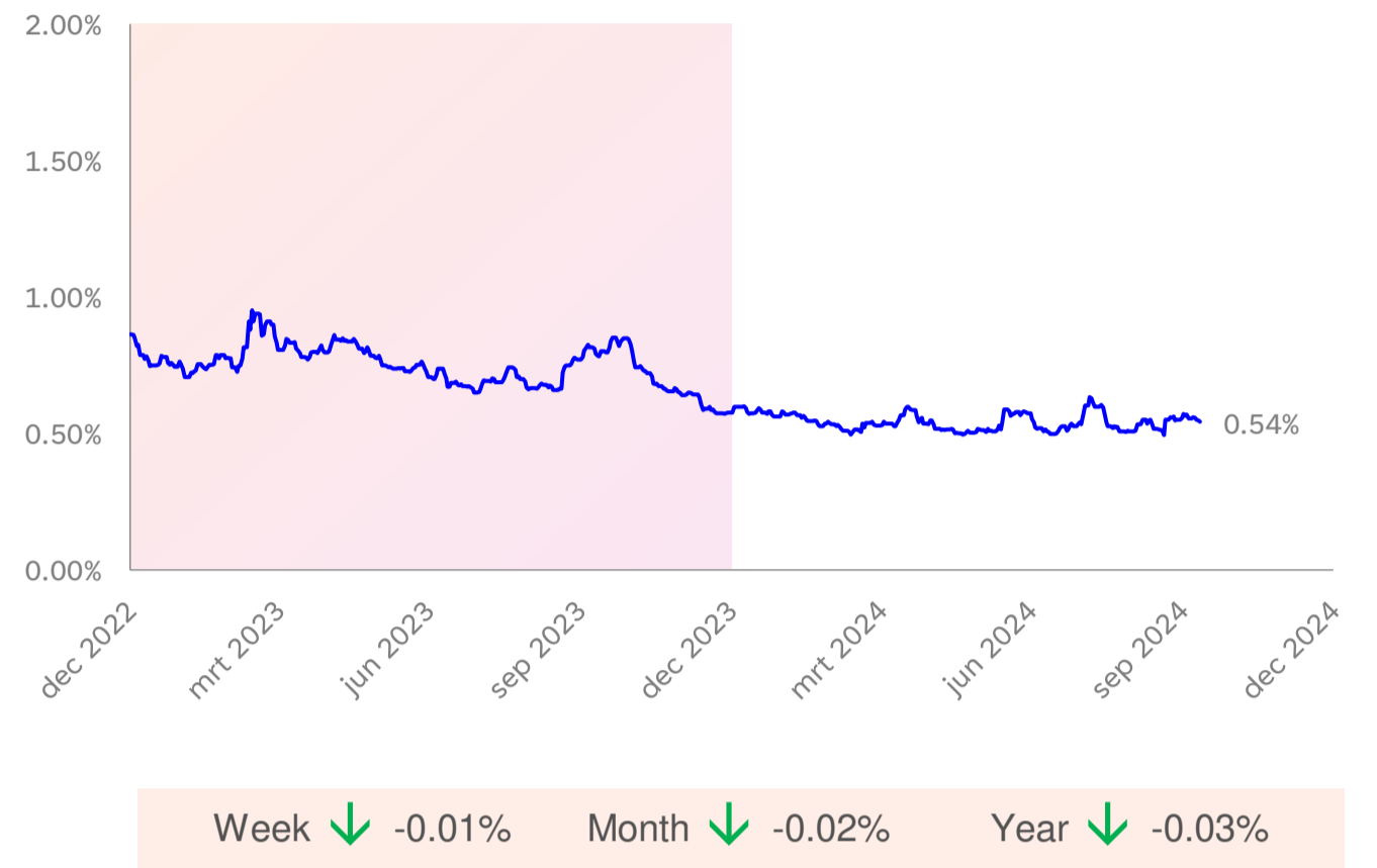
Figure 2: Credit risk
