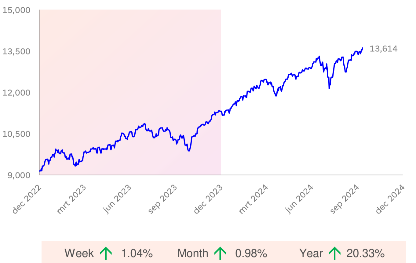
Figure 4: Equity risk
