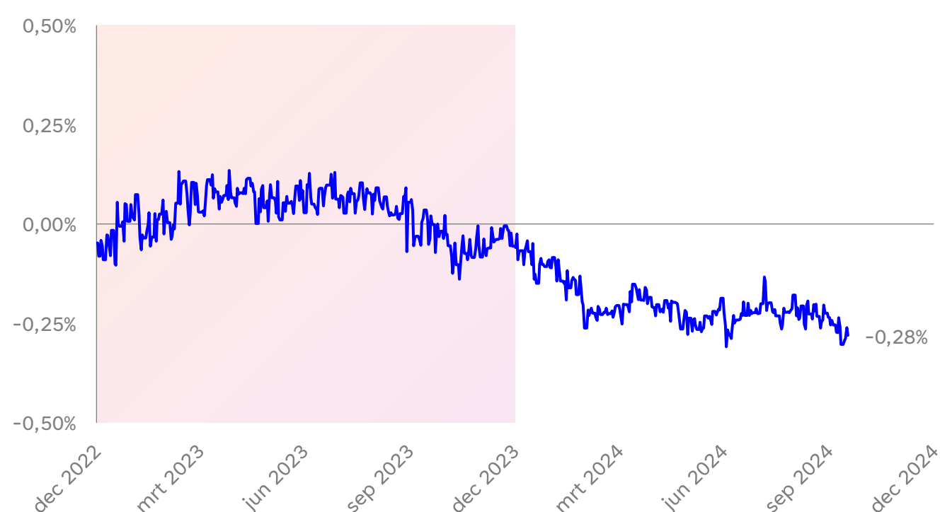
Figuur 5: Swapspreadriscio
