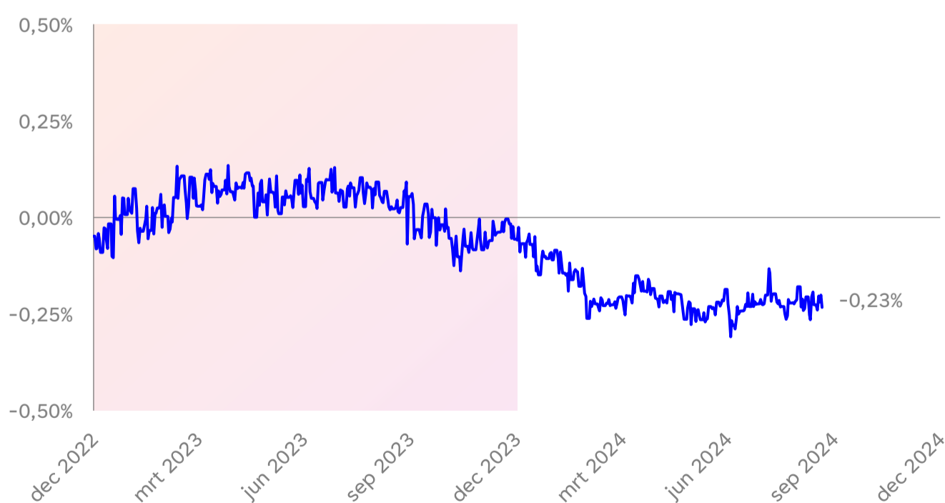
Figuur 5: Swapspreaddrisico
