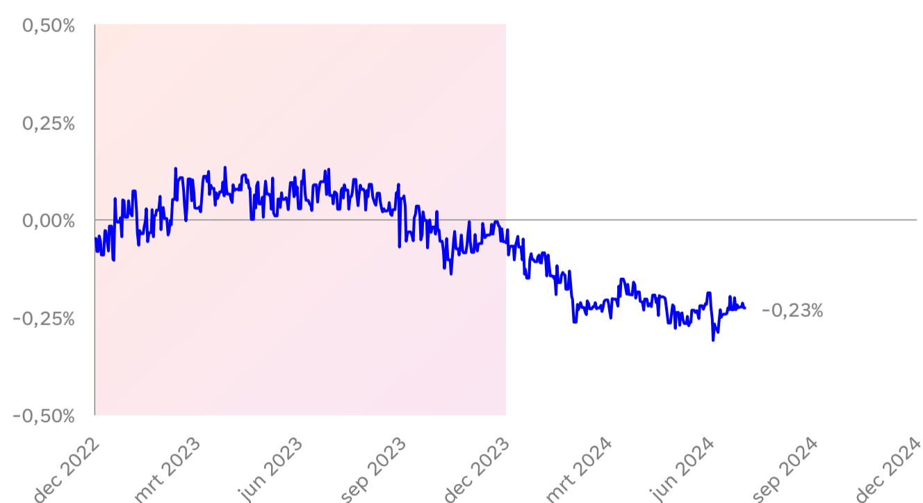
Figuur 5: Swapspreaddrisico
