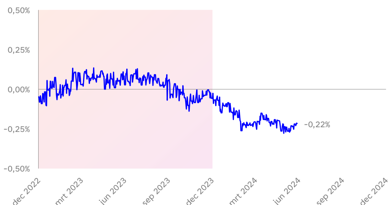
Figuur 5: Swapspreadriscico
