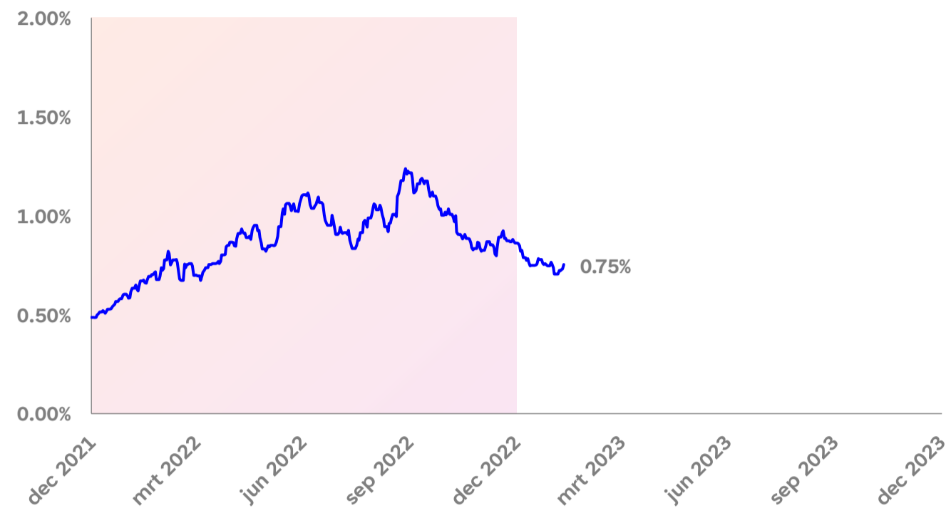
Figure 2: Credit risk
